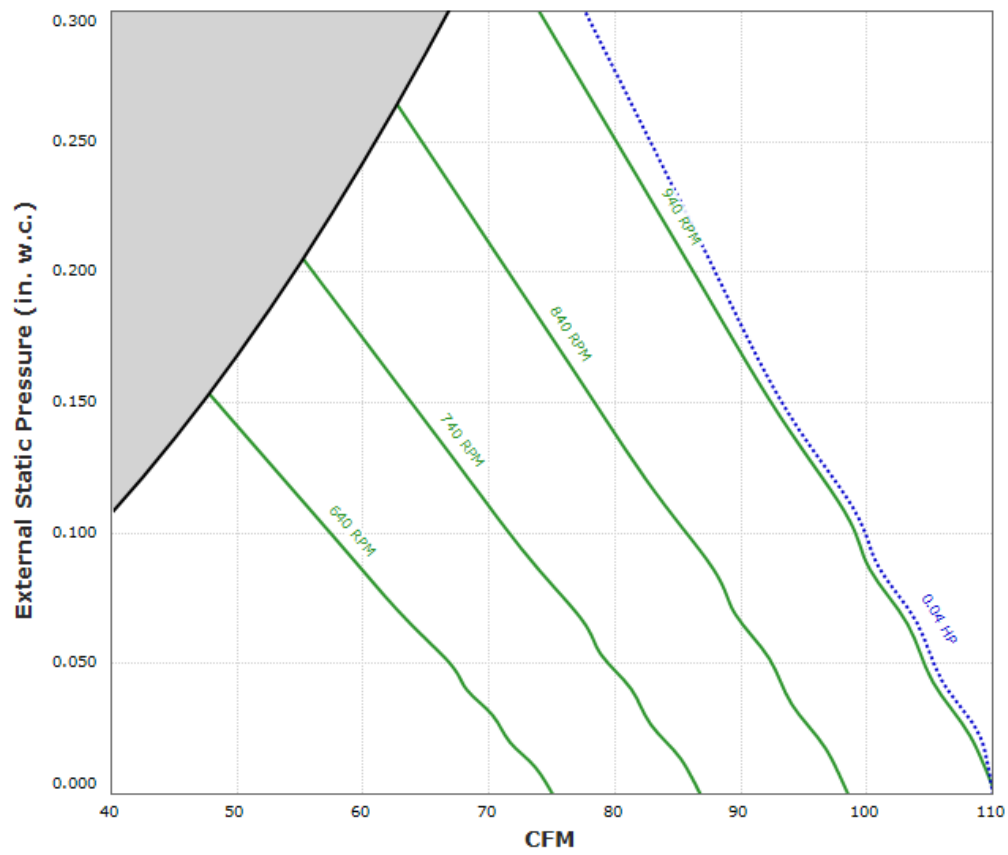
CFA-S90-RA Performance Curve
